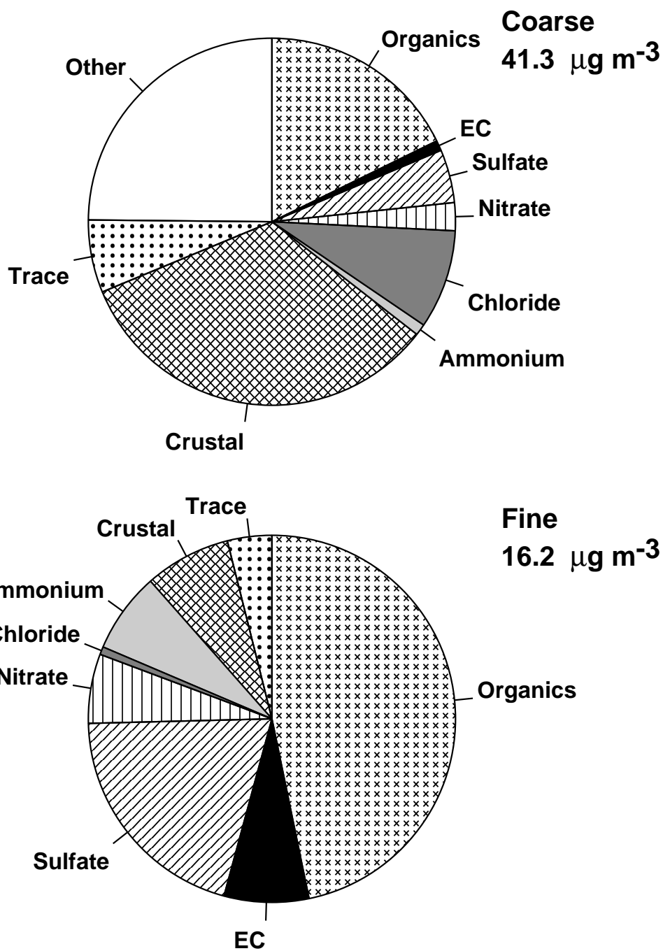
Figure 3.1 - Coarse and Fine Particle Chemical Composition, 1995 Annual Average - Kenmore Square, Boston, MA
